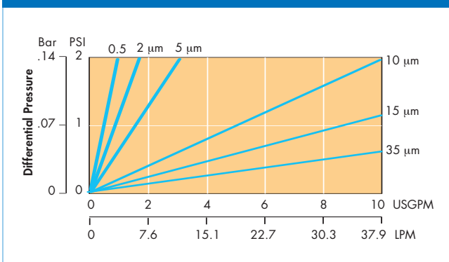
TPM 2.36" (60mm) WATER FLOW RATES
