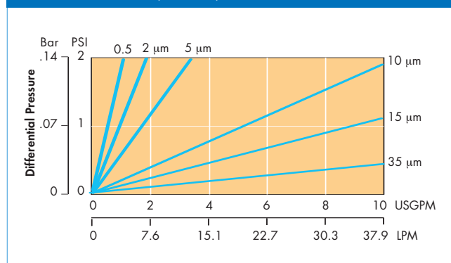
TPM 2.75" (70mm) WATER FLOW RATES
