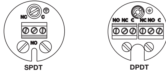
TERMINAL CONNECTIONS
